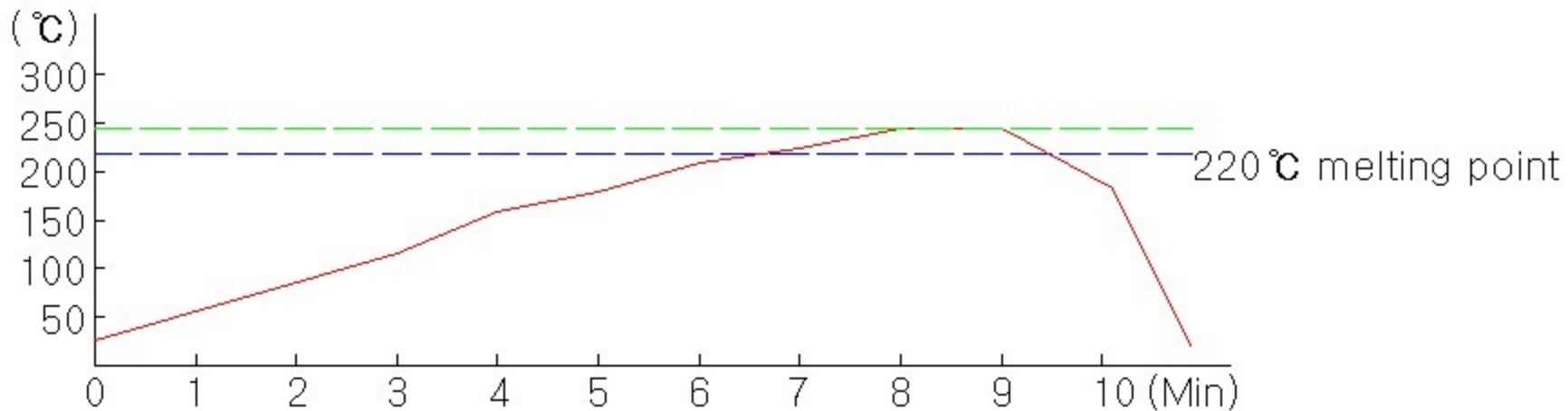
4R3P, 4R4P, 4R10P solder reflow profile (Sn-Ag-Cu 계)
